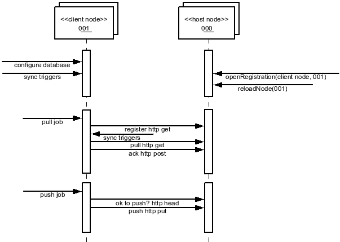
Figure 4.1. Node Communication
